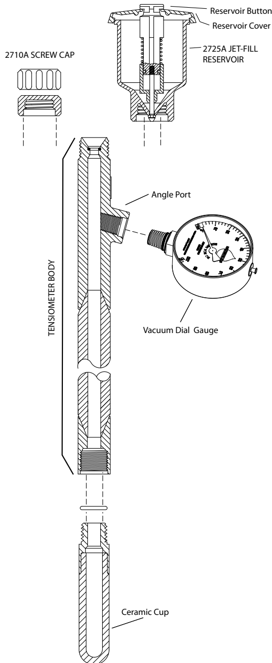
(Fig. 2) 2710ARL and 2725ARL Tensiometer Parts
