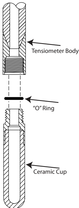
(Fig. 4) Attaching the Ceramic Tip
