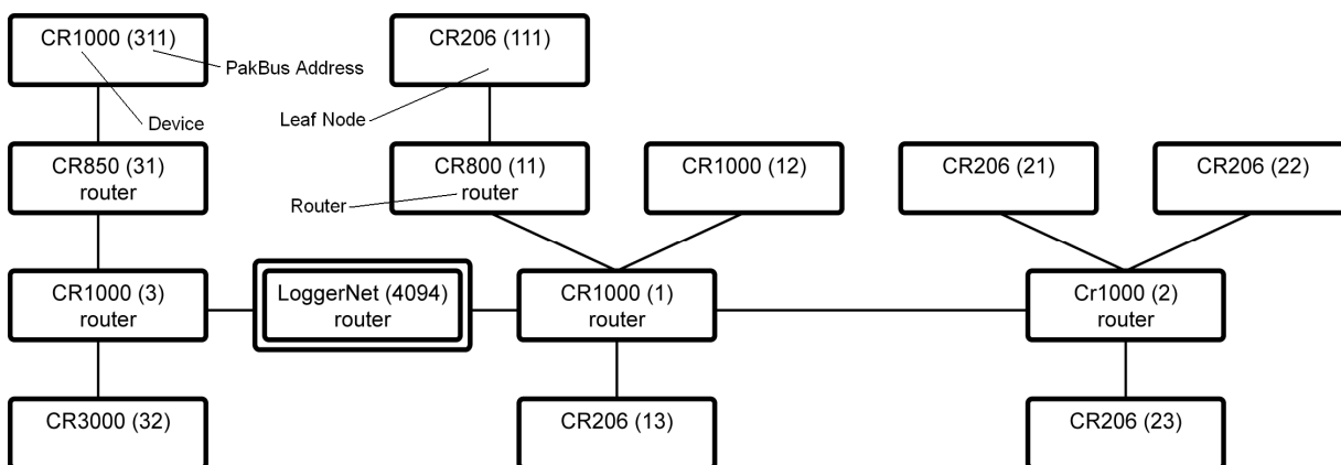
Figure 49: PakBus Network Addressing.
