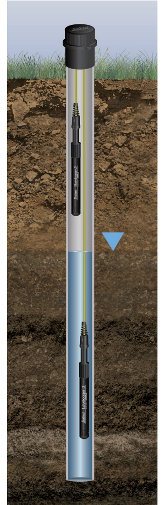
Barologger 5 and Levelogger 5 installed in Well Using L5 Direct Read Cables
